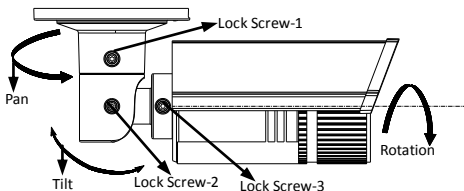
Figure 2-8 Lens Adjustment
